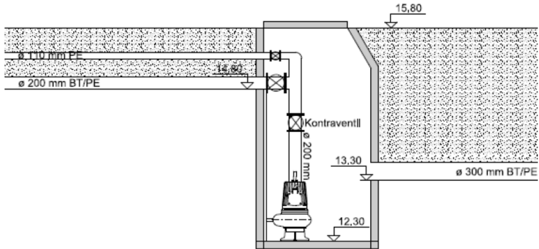
Figur 9.1 Design af pumpestation
